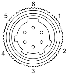
View is from front of mating connector
