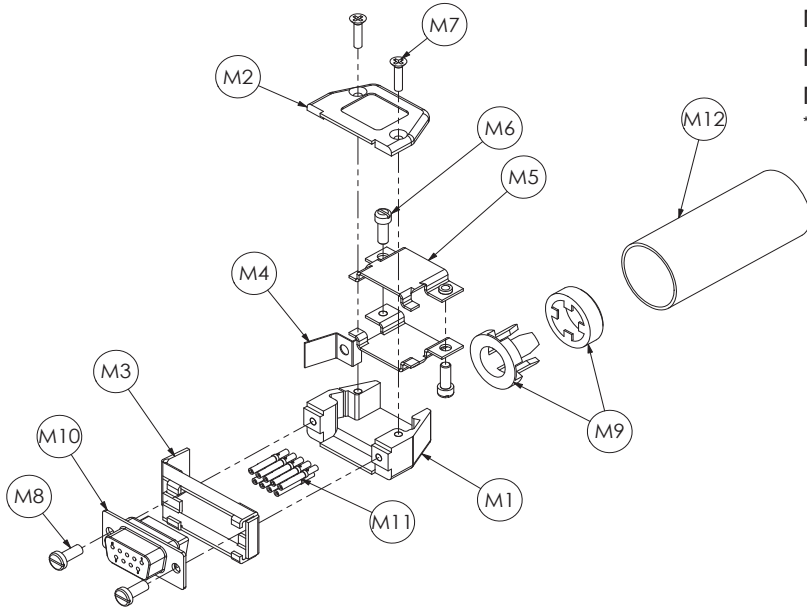
9 Pin Connector Assembly
