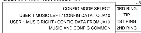
JA10-070 MUSIC CONFIGURATION CONNECTOR
